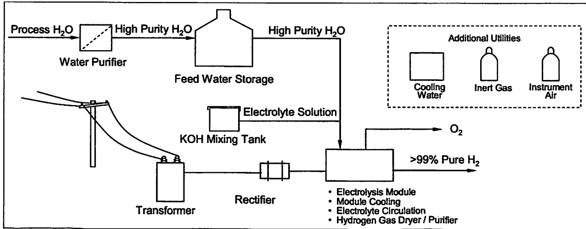
Figure 1. Electrolysis process flow diagrams
