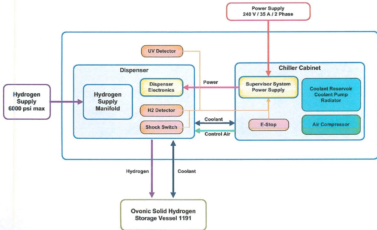
Fig. 2. Hydrogen Dispensing System – Block diagram
